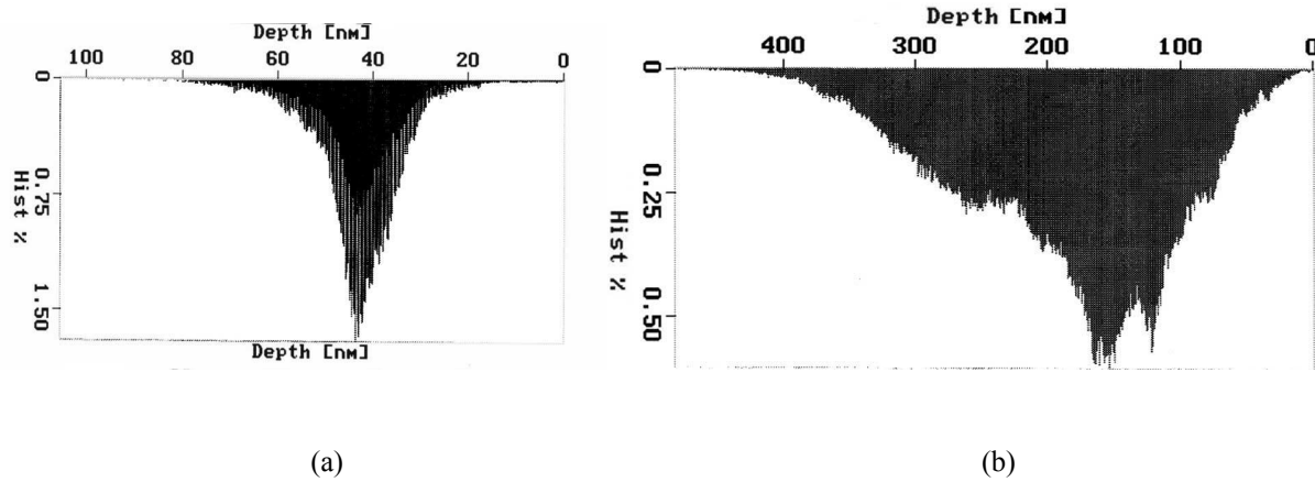
Fig 2...Atomic Force Microscopy of Laser-treated Cartilage: (a) intact cartilage, (b) laser treated cartilage
